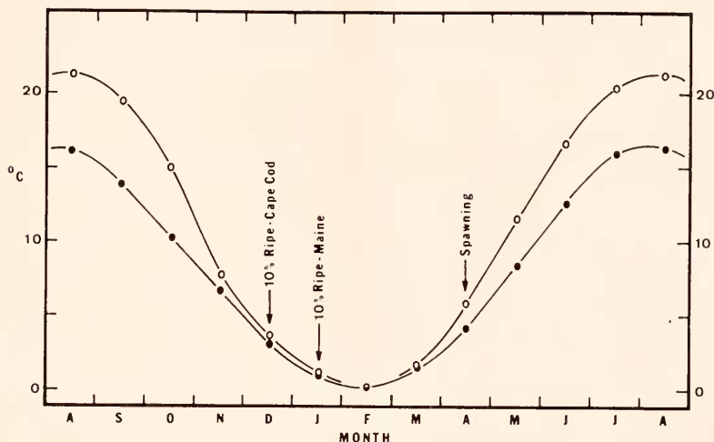
FIGURE 1. Mean monthly sea temperature for Boothbay Harbor, Maine (filled circles) and for Woods Hole, Massachusetts (open circles); from the data of Taylor, Bigelow, and Graham, 1957.
